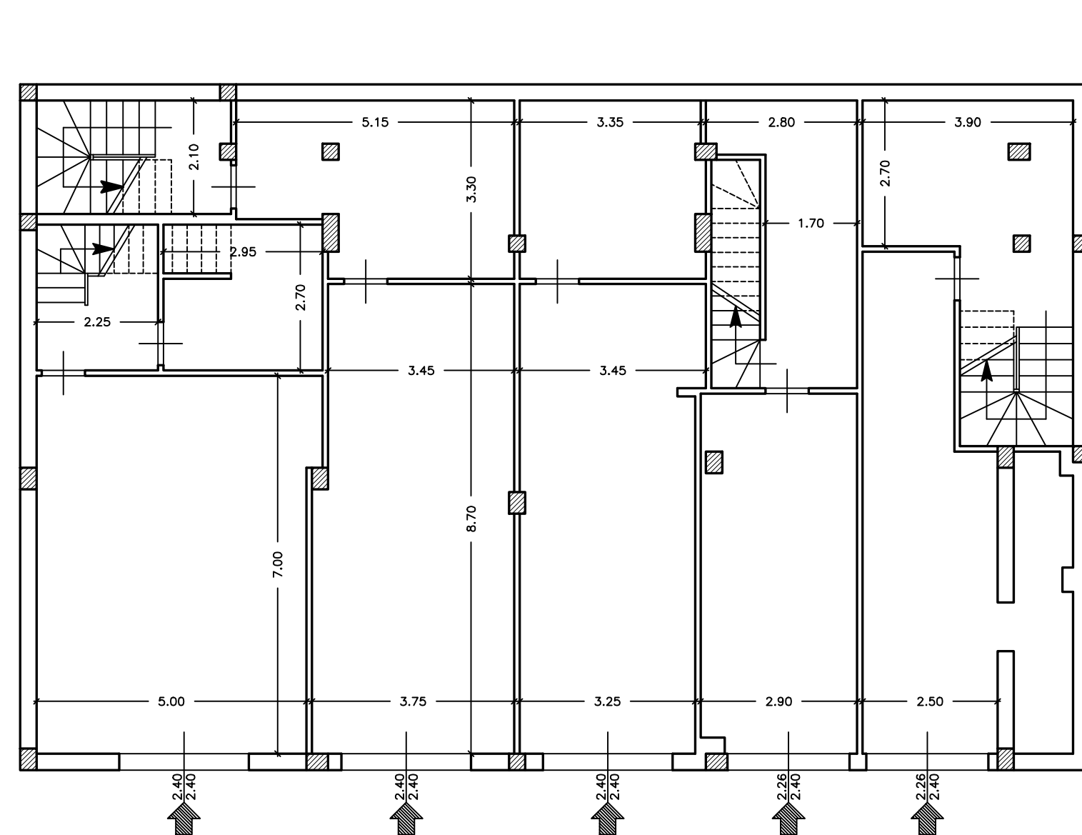
PIANO INTERRATO
