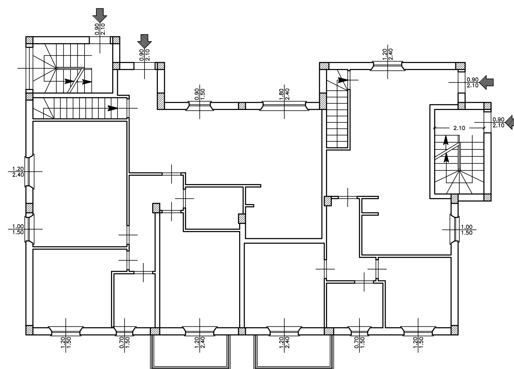
PIANO TERRENO
